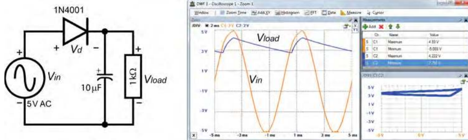
Figure 4-10: Circuit and behavior of a 1N4001 diode with a 5V AC supply, 1\text{k}\Omega load, and parallel 10\mu\text{F} capacitor
