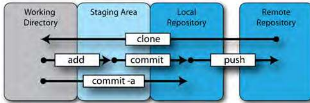
Figure 3-4: The basic Git workflow
