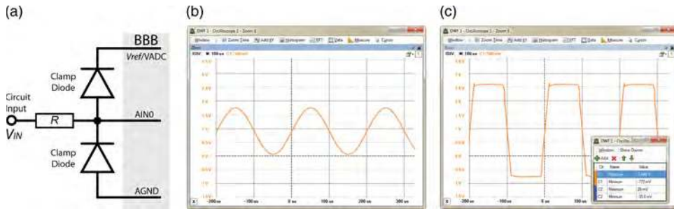
Figure 9-9: (a) A typical diode clamping circuit (not recommended); (b) the signal response of the circuit to an input signal that is in range; (c) the clipped signal response of the circuit to an input signal that is out of range
