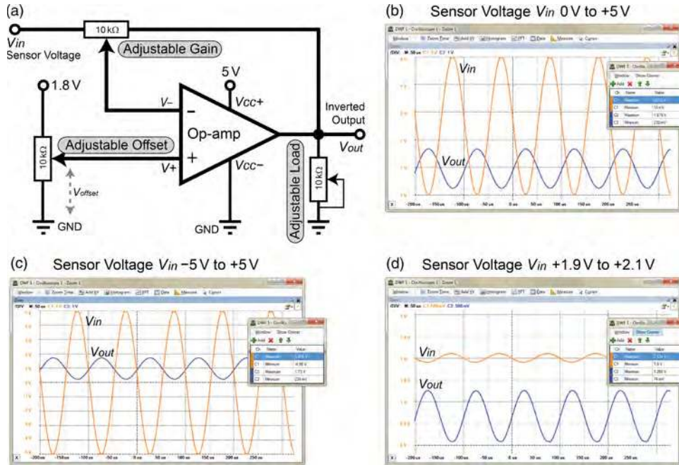
Figure 9-12: (a) A general op-amp signal conditioning circuit that inverts the input; (b) conditioned output when V_{in} is 0V to 5V; (c) output when V_{in} is -5V to +5V; (d) conditioned and amplified output when the input signal is 1.9V to 2.1V
