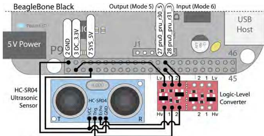
Figure 13-11: The HC-SR04 ultrasonic distance sensor circuit
