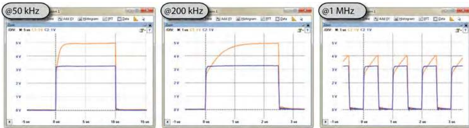
Figure 8-20: Switching BSS138-based translators from 3.3V to 5V logic levels at 50kHz, 200kHz, and 1MHz
