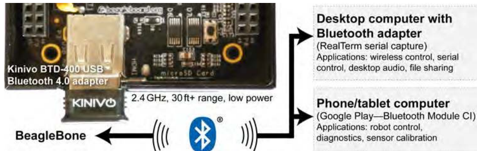
Figure 9-23: Bluetooth-connected BeagleBone
