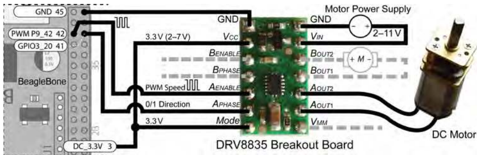
Figure 9-3: Driving a DC motor using an example H-Bridge driver breakout board
