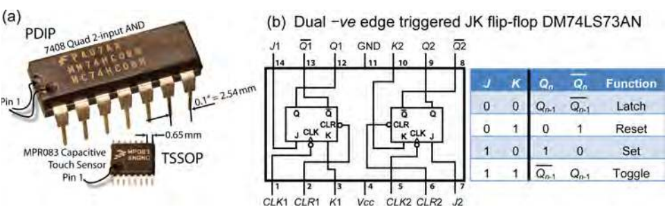
Figure 4-22: (a) IC package examples (b) The JK flip-flop
