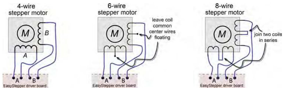
Figure 9-6: Wiring configuration for different stepper motor types
